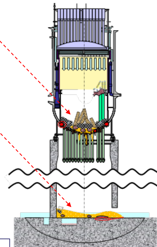
Assumed Fuel Debris Distribution (1F-2)*
