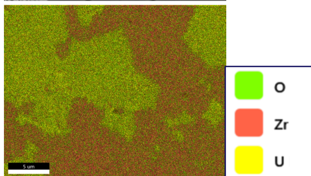
切削試験前試料断面SEM-EDS
