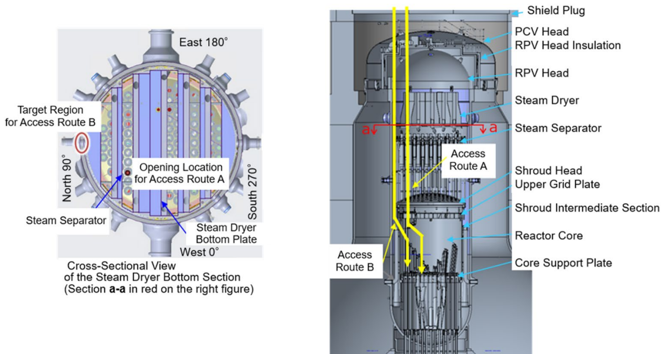
Figure 2 Proposed Access Routes for Access-from-Top Investigation through Small-Diameter Top Opening
