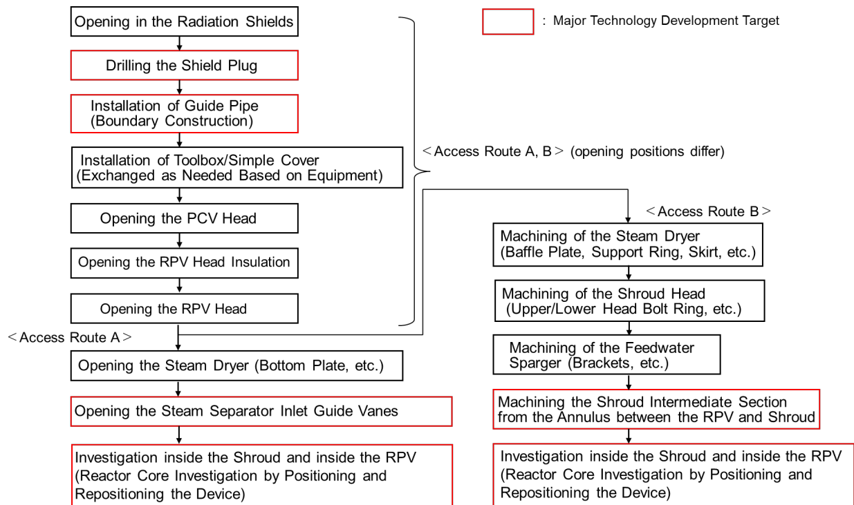
Figure 3 Work Steps for the Access-from-Top Investigation through Small-Diameter Top Opening (Proposed Access Routes A and B)
