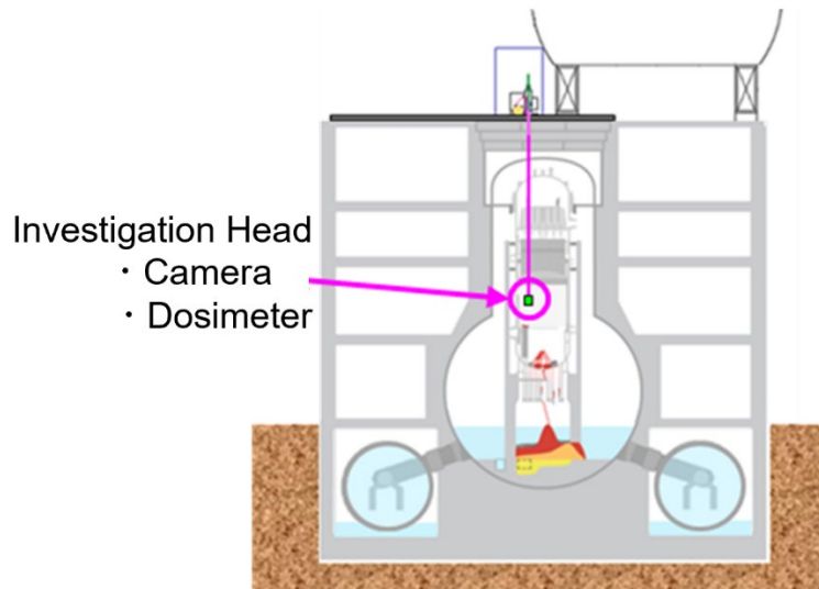
Figure 1: Conceptual Image of Access-from-Top Investigation through Small-Diameter Top Opening Source: “Design Study on Fuel Debris Retrieval for Unit 3,” July 31, 2025, meeting documents of the Secretariat of the Team for Decommissioning, Contaminated Water and Treated Water Countermeasures / PMO
